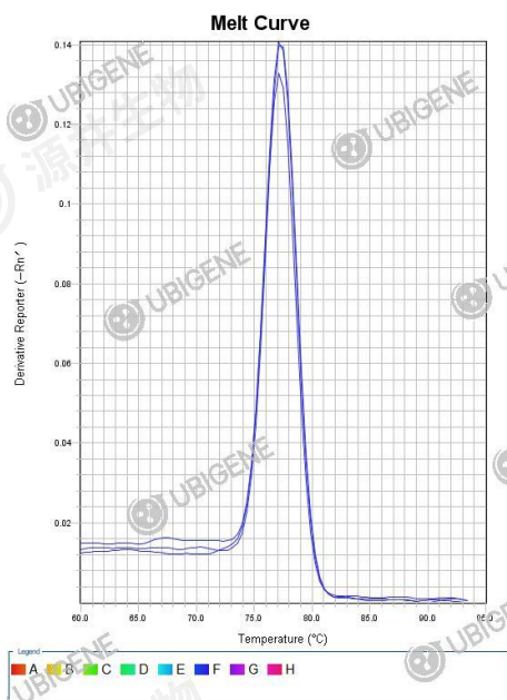
Huh-7_Ctrl(Puro)+hNAE1-1 melt curve
