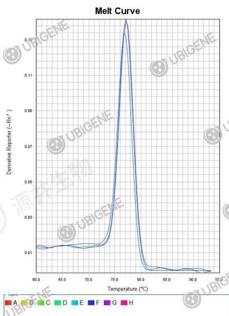
NAE1 Stable Expression Cell Line (HuH-7)+hNAE1-1 melt curve
