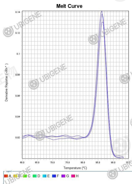
Huh-7_Ctrl(Puro)+ \beta -h_actin melt curve
