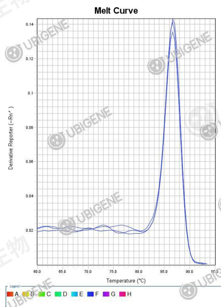
NAE1 Stable Expression Cell Line (HuH-7)+ \beta -h_actin melt curve
