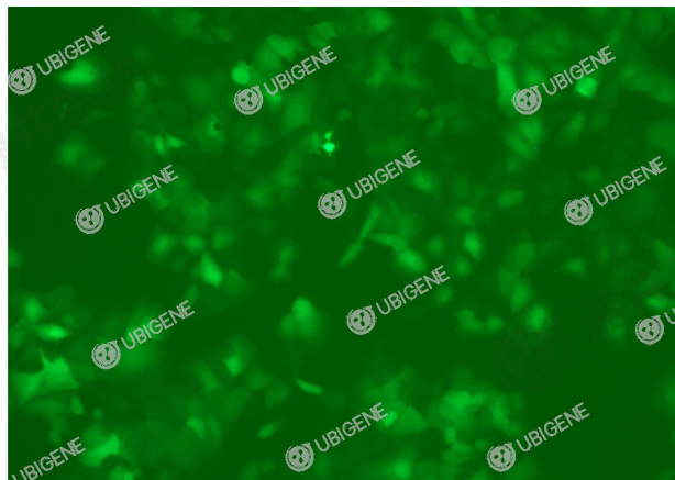
NAE1 Stable Expression Cell Line (HuH-7)-100X- 300ms
