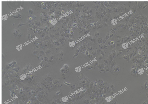
NAE1 Stable Expression Cell Line (HuH-7)-100X
